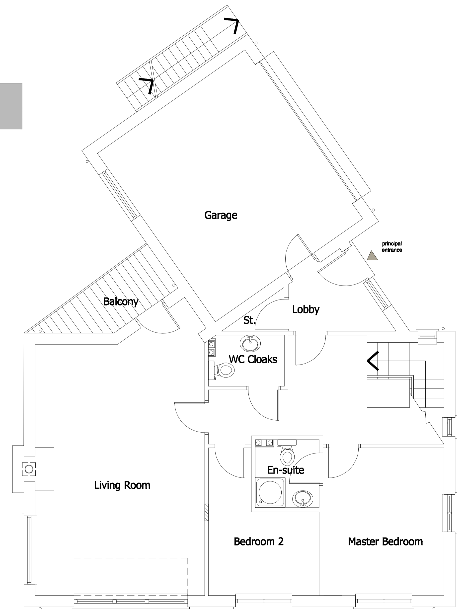
Ground Floor Plan(upper level)+Roof Plan
