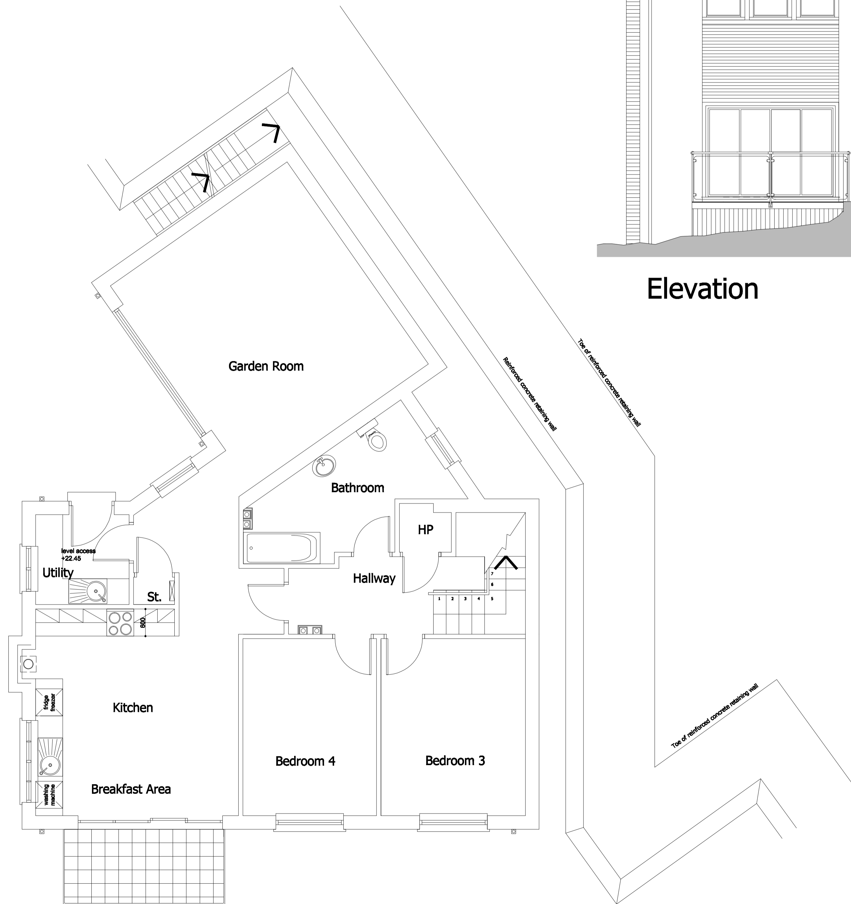
Ground Floor Plan(lower level)
